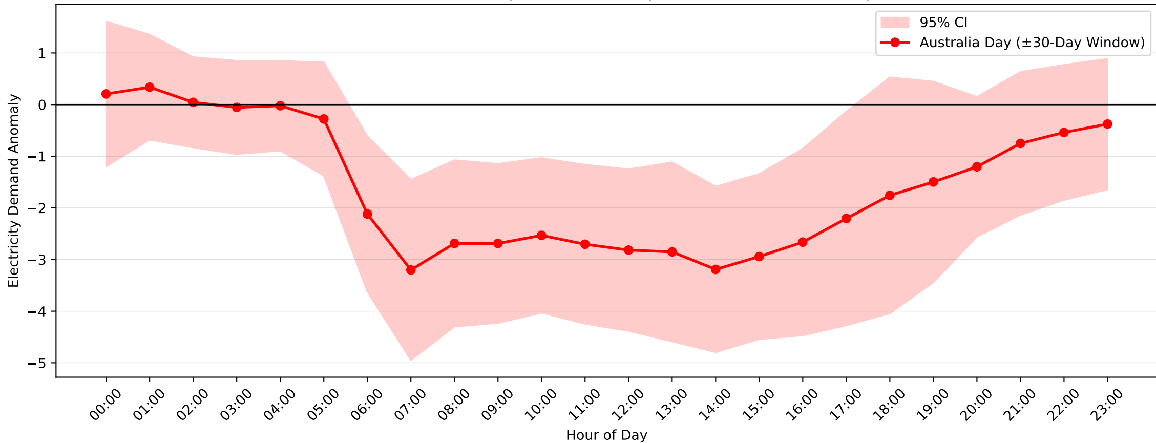
Matravlle Demand Anomaly: Australia Day (2004-2017, \pm 30 -Day Window)
